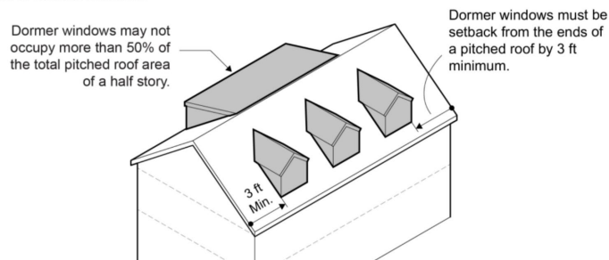
Figure 7. Dormer Windows
